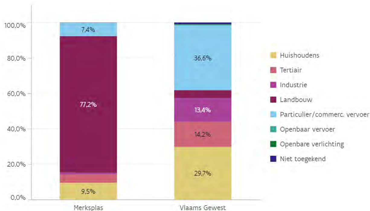
CO 2 -emissies per sector, 2019, in procenten
